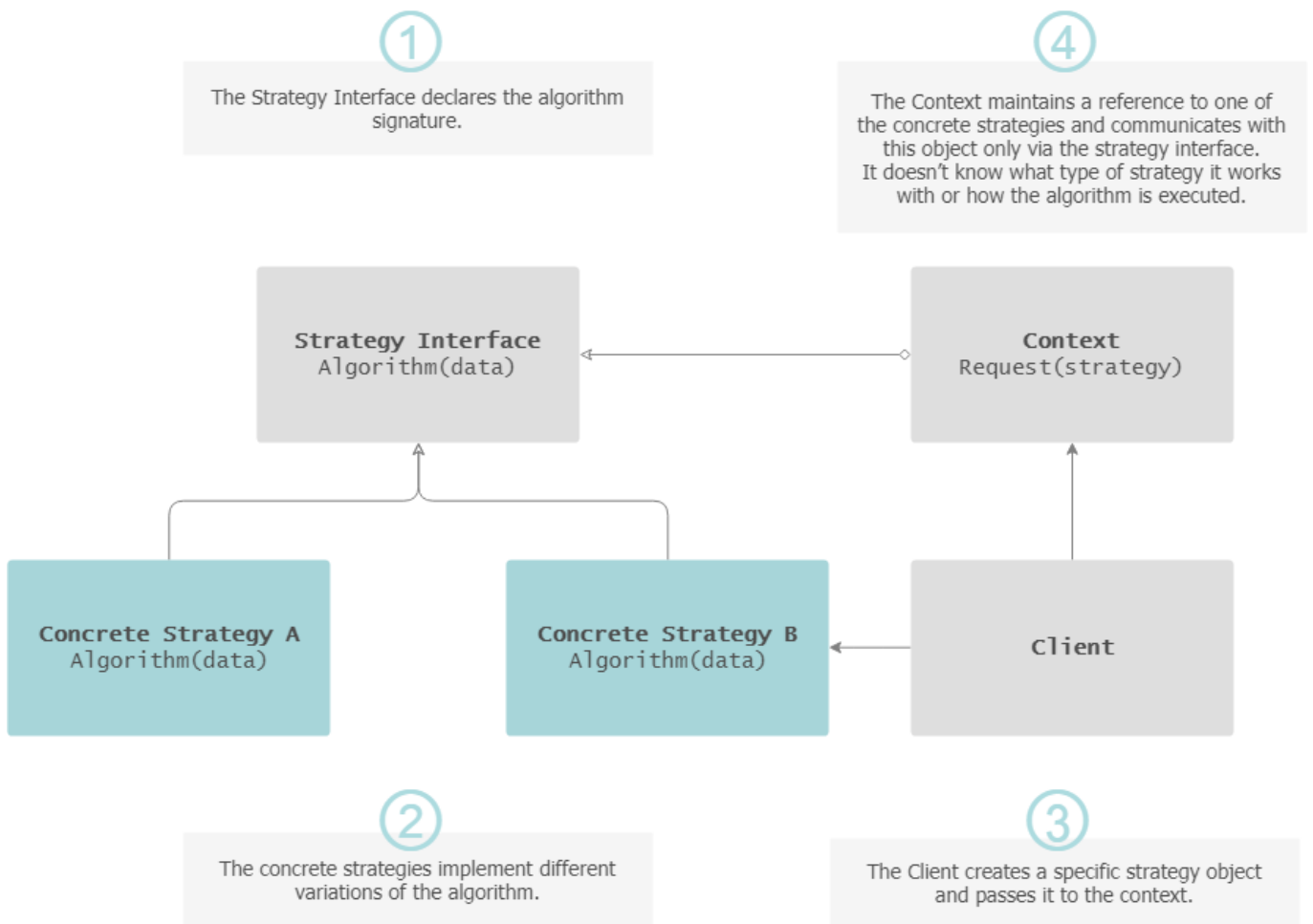
Strategy Pattern
