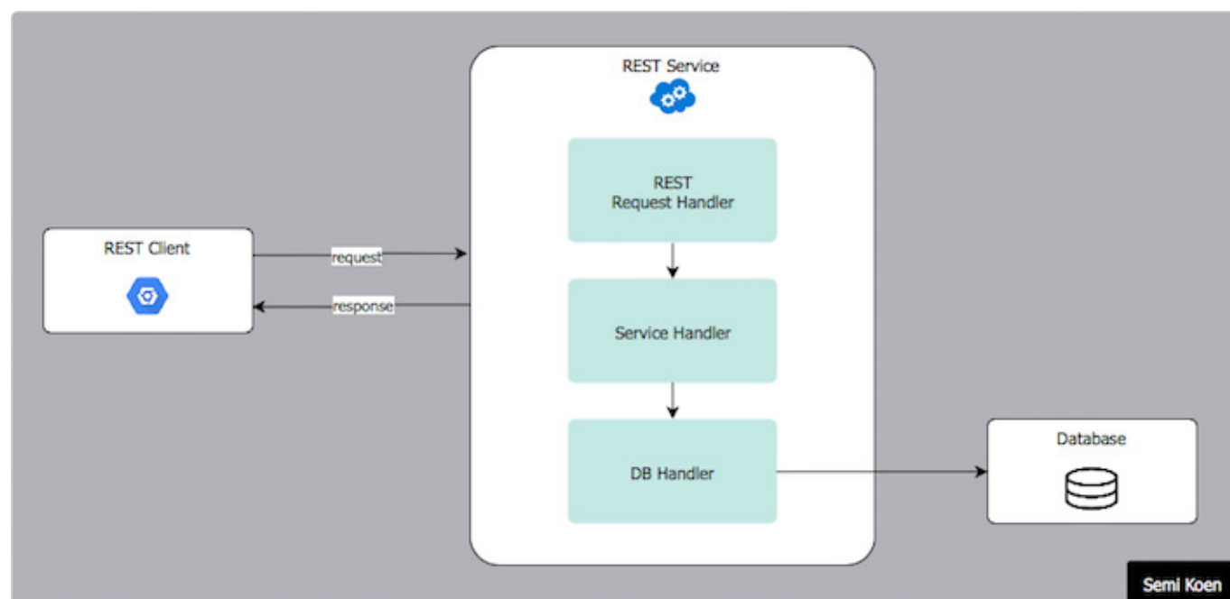
REST Architecture
