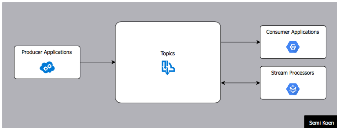
Streaming Architecture
