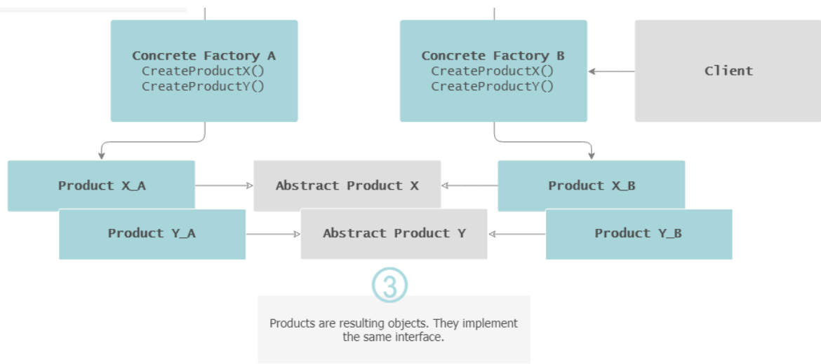
Abstract Factory
