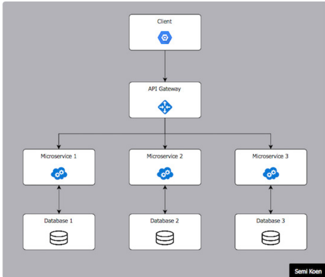
Microservices Architecture
