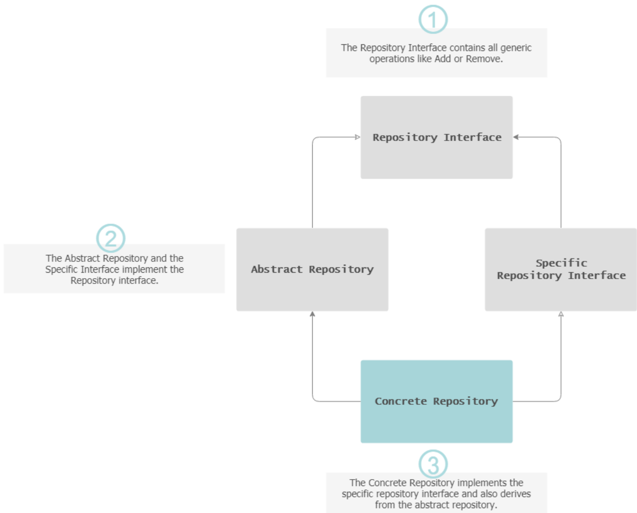
Repository Pattern
