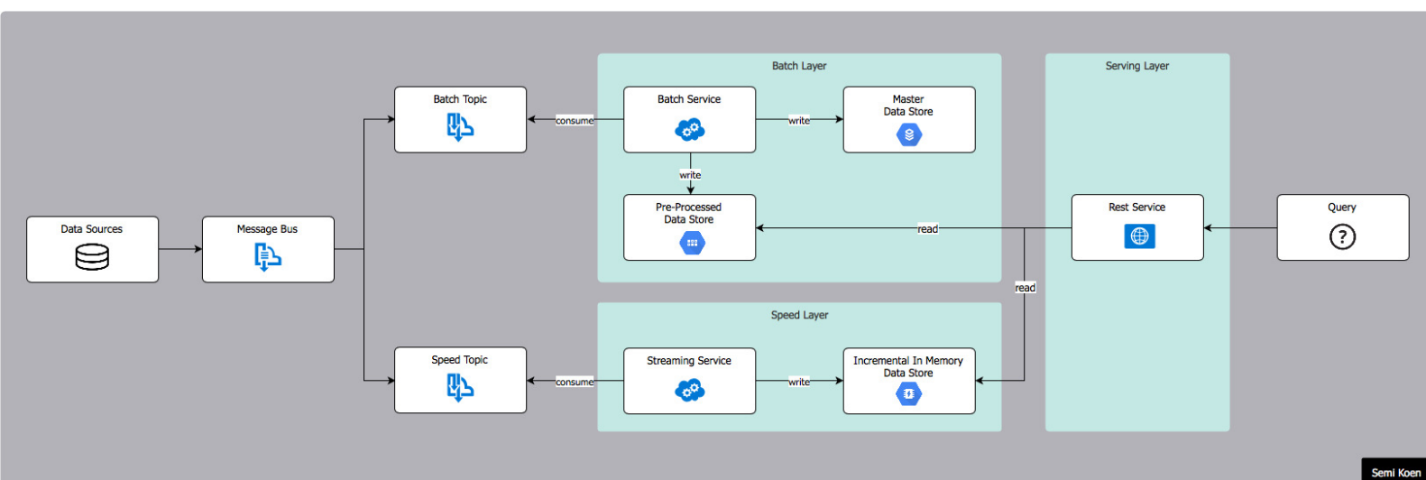
Lambda Architecture
